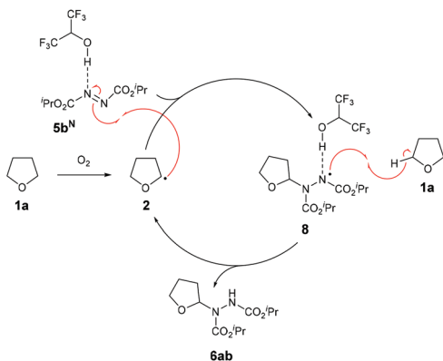
Scheme 5 Proposed mechanism.
