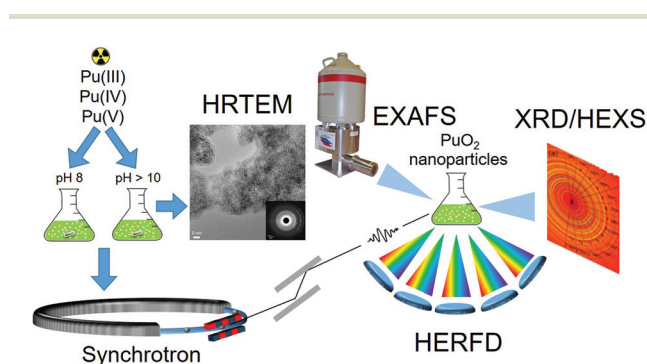
Fig. 1 The schematic illustration of the research methodology applied to \text{PuO}_2 NPs studies. \text{PuO}_2 NPs synthesized from different precursors (Pu(III), Pu(IV) and Pu(V)) and at pH 8 and pH > 10 were analysed with HRTEM and various synchrotron techniques (EXAFS, XRD, HEXS and HERFD).
