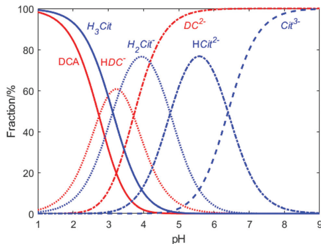
Fig. 11 Relative concentration of the different dissociation species of sodium citrate and DCA as a function of pH. H_3Cit , H_2Cit^- , HCit^{2-} and Cit^{3-} represent different forms of citrate. DCA, HDC^- and DC^{2-} represent different forms of dicarboxyacetone (according to reactions (3) and (4)). The pK_a values for citrate hydrolysis are 3.1, 4.76, 6.4, respectively; the pK_a values for dicarboxyacetone are 2.74 and 3.72 respectively.
