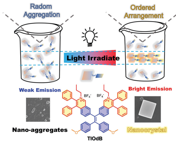
Scheme 1 Illustration of the photoexcitation process and molecular structures of TIOdB.
