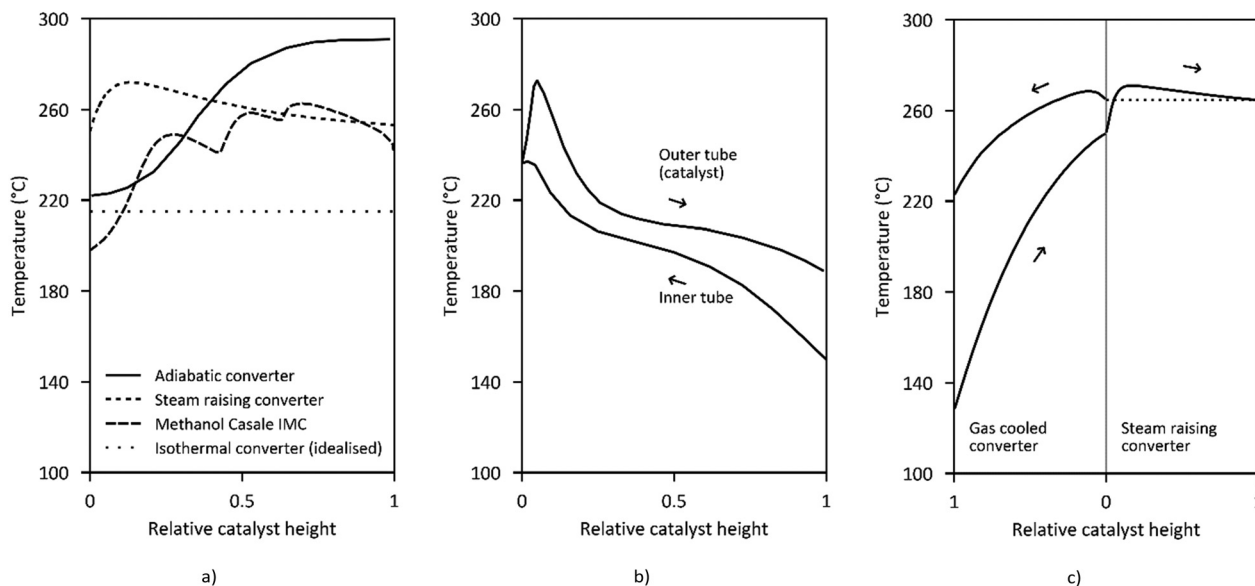
Fig. 7 Temperature profiles along the reactor length of (a) adiabatic converter, 105 steam raising converter, 126 Methanol Casale IMC, 142 and isothermal converter (idealised), (b) Mitsubishi Superconverter, 143 (c) Lurgi MegaMethanol. 99
