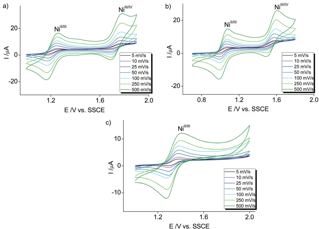
Fig. 6 Cyclic voltammetry measurements of homoleptic [\text{Ni}(\text{pyPYA}_2)_2](\text{PF}_6)_2 complexes in MeCN: (a) 3a [\text{Ni}(\textit{para}\text{-pyPYA}_2)_2](\text{PF}_6)_2 ; (b) 3b [\text{Ni}(\textit{meta}\text{-pyPYA}_2)_2](\text{PF}_6)_2 ; (c) 3c [\text{Ni}(\textit{ortho}\text{-pyPYA}_2)_2](\text{PF}_6)_2 . Conditions: 10 mL solvent, 1 mM sample and 100 mM (n\text{Bu}_4\text{N})\text{PF}_6 as supporting electrolyte at 5–500 \text{mV s}^{-1} scan rate (potentials vs. SSCE using the \text{Fc}^+/\text{Fc} couple as standard; E_{1/2} = +0.4319 ).
