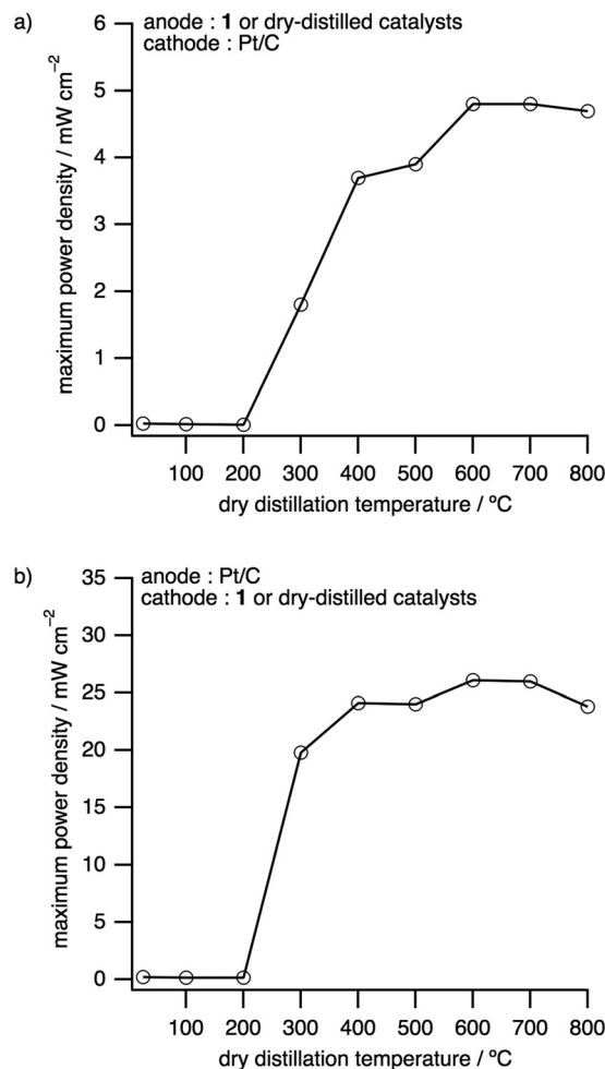
Fig. 5 Maximum power densities of \text{H}_2 -O 2 fuel cells depending on the dry distillation temperature. At the dry distillation temperature of 25 °C, 1 is used as it is as a fuel cell catalyst. (a) Anode: 1 or DDCs. Cathode: Pt/C. (b) Anode: Pt/C. Cathode: 1 or DDCs.
