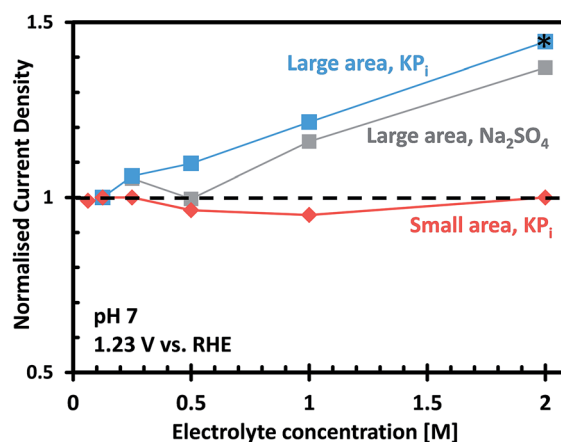
Fig. 6 Normalized photocurrent measured at 1.23 V_{\text{RHE}} under AM 1.5G illumination, for the small and large CoP i /W:BiVO 4 photoanodes as a function of concentration of electrolyte (pH 7). Zero concentration corresponds to pure deionized water. *Electrolyte selected for all measurements using the large area BVO 4 without hole scavenger.
