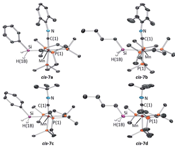
Fig. 7 X-ray crystal structures of (top left) cis -[(dmpe) 2 Mn(SiH 2 -Ph)(CN x yllyl)] ( cis -7a), (top right) cis -[(dmpe) 2 Mn(SiH 2 t Bu)(CN x yllyl)] ( cis -7b), (bottom left) cis -[(dmpe) 2 Mn(SiH 2 Ph)(CN t Bu)] ( cis -7c), and (bottom right) cis -[(dmpe) 2 Mn(SiH 2 t Bu)(CN t Bu)] ( cis -7d), with ellipsoids drawn at 50% probability. Most hydrogen atoms have been omitted for clarity. cis -7c and cis -7d crystallized with two independent and essentially isostructural molecules in the unit cell, only one of which is shown. All structures exhibit some disorder, and only the dominant conformation is shown.
