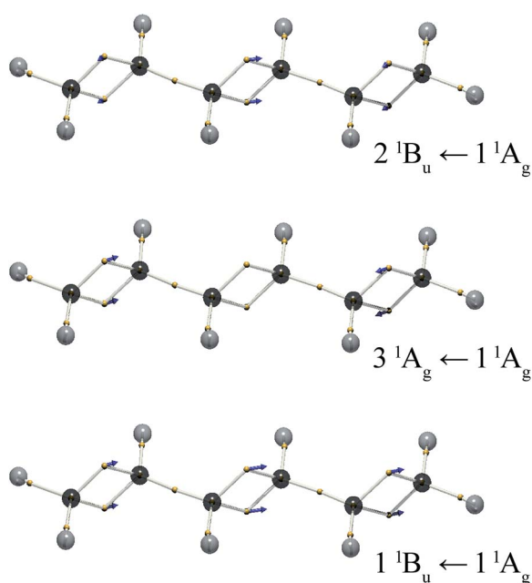
Fig. 6 The electron positions for the mid-point of the vibration, x = (x_i + x_f)/2 , and the displacement vectors x_{ri} , for the 1^1B_u \leftarrow 1^1A_g , 3^1A_g \leftarrow 1^1A_g and 2^1B_u \leftarrow 1^1A_g transitions of trans,trans -hexatriene. The vector length is doubled for clarity.
