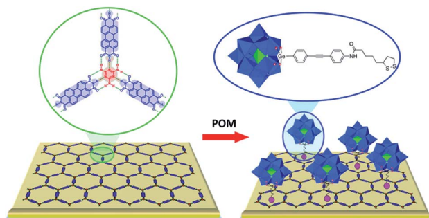
Fig. 13 Schematic depiction of the organisational preferences of the Keggin-type POM-based inorganic-organic hybrid units [PW_{11}O_{39}Ge(p-C_6H_4-C\equiv C-C_6H_4-NHC(O)(CH_2)_4(-CH-(CH_2)_2S-S-))_4]^{4-} (right) on the PTCDI/melamine-templated gold surface (left). Colour code: W, blue; P, green polyhedra; O, red spheres. Adapted with permission from ref. 29. Copyright 2016 American Chemical Society.
