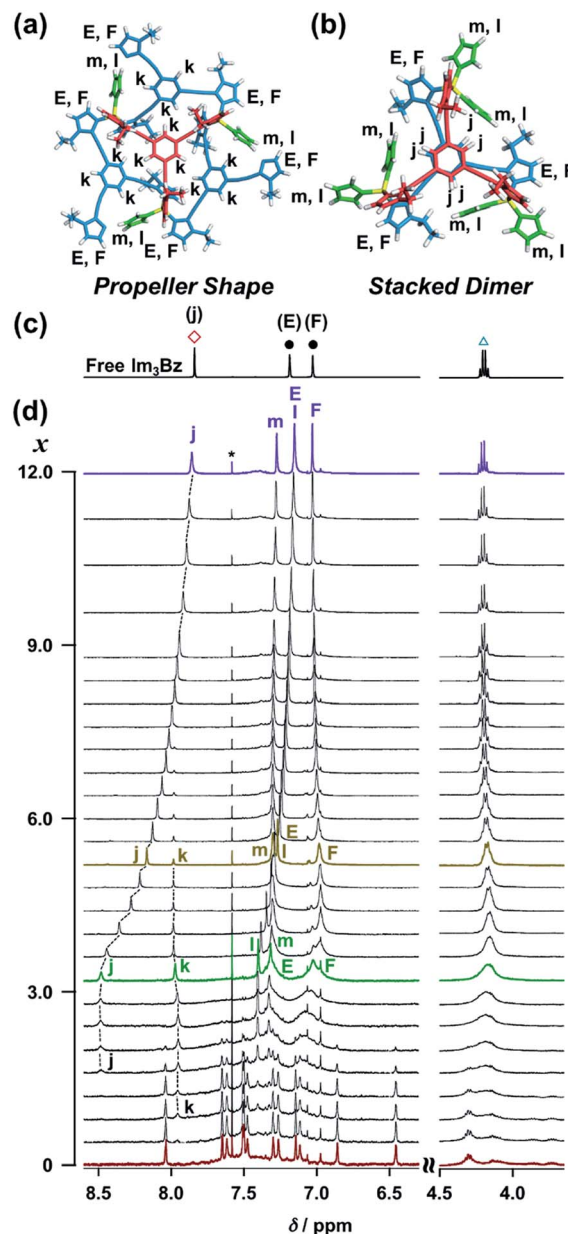
Fig. 7 Energy minimized structures and NMR signal assignment of (a) (\text{ImH}_2)_3(\text{Im}_3\text{Bz})_4(\text{Zn}^{2+})_3 and (b) (\text{ImH}_2)_6(\text{Im}_3\text{Bz})_2(\text{Zn}^{2+})_3 . (c) ^1\text{H} NMR spectrum of free \text{Im}_3\text{Bz} ( 1.8 \times 10^{-3} M) in \text{CD}_3\text{CN} , where symbols correspond to those in the chemical structure \text{Im}_3\text{Bz} (Fig. 3). (d) Stacked ^1\text{H} NMR spectra of \text{Im}_3\text{Bz} ( 1.8 \times 10^{-3} M) with \text{Zn}^{2+} ( 1.4 \times 10^{-3} M) in the presence of \text{ImH}_2 ( 0 – 5.4 \times 10^{-3} M, 0: red line, 1.4 \times 10^{-3} M: green line, 2.3 \times 10^{-3} M: yellow line, and 5.4 \times 10^{-3} M: purple line) in \text{CD}_3\text{CN} at 298 K ( x = [\text{ImH}_2]/[(\text{Im}_3\text{Bz})_4(\text{Zn}^{2+})_3]_0 ). Asterisk denotes chloroform.
