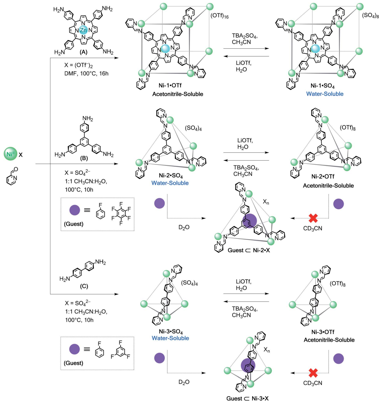
Scheme 2 Subcomponent self-assembly of water-soluble Ni-1 \cdot SO_4 to Ni-3 \cdot SO_4 cages from anilines A–C, their reversible anion-exchange sequences and encapsulation of selected fluorinated guests.
