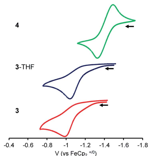
Fig. 3 CVs of 3 , 3-THF and 4 with 0.1 M [ ^n\text{Pr}_4\text{N} ][ \text{BAR}_4^{\text{F}} ] electrolyte in DFB (scan rate of 100 mV s ^{-1} ; collected under Ar).
