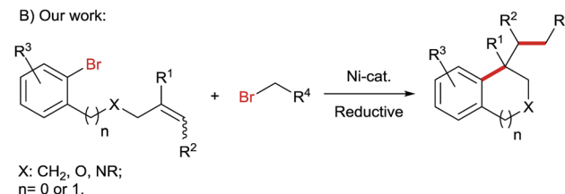
Scheme 1 Redox-neutral (A) and reductive (B) arylalkylation of tethered alkenes for the synthesis of benzene-fused cyclic compounds.
