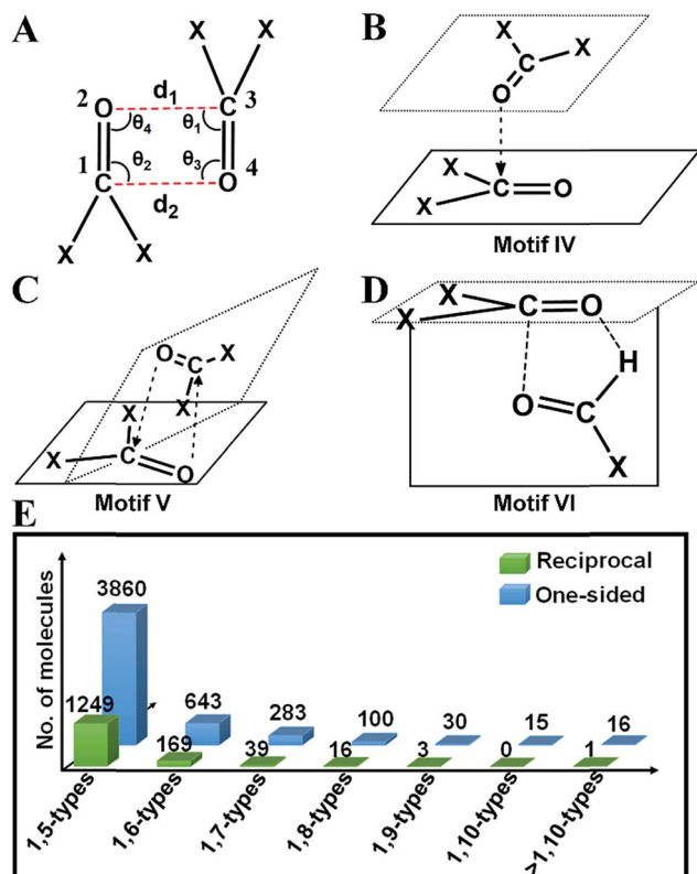
Fig. 4 Chemical structures of some motifs newly discovered in this study. (A) Fragment having \text{C}=\text{O}\cdots\text{C}=\text{O} short contacts used for the CSD search. Torsion angle, T is defined as \text{C}^1=\text{O}^2\cdots\text{C}^3=\text{O}^4 . Chemical structures of newly discovered (B) motif IV (C) motif V and (D) motif VI. (E) Plot showing how the number of molecules decreases for intra-molecular one-sided and reciprocal interactions as the bond separation between the two carbonyl groups increases. In 1,x -type interaction x represents the size of the ring to be formed due to the interaction. For example, 1,5-type interaction means there are 3 bonds separating the carbonyl groups and a 5-membered ring will be formed due to the noncovalent interaction.
