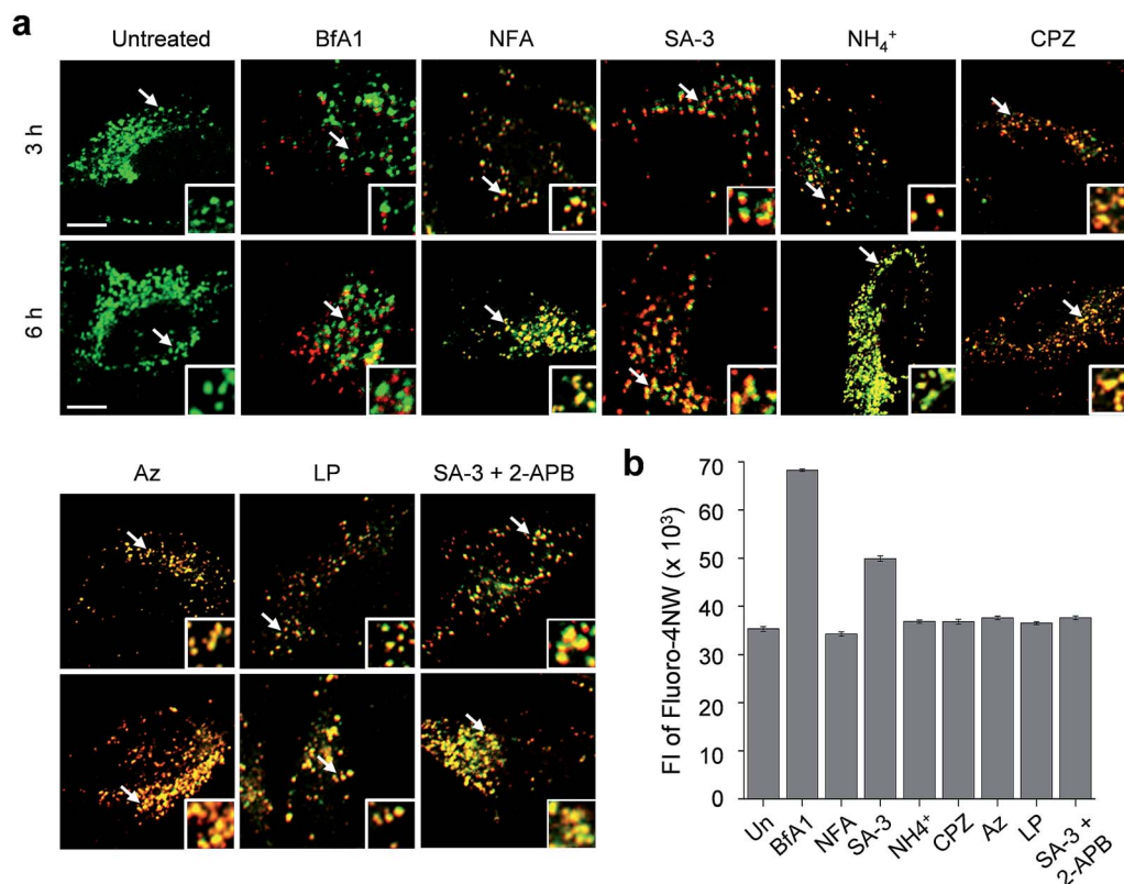
Fig. 7 Effect of substances on the fusion of autophagosomes with lysosomes. (a) HeLa cells were incubated for 3 or 6 h with an individual compound (200 nM BfA1, 5 μM NFA, 5 μM SA-3, 30 mM NH 4 + , 20 μM CPZ, 5 μM Az, 50 μM LP, and 5 μM SA-3 + 10 μM 2-APB). The cells were immunostained with LAMP2A and p62 antibodies. Merged images of the cells immunostained with LAMP2A and p62 antibodies are shown (scale bar: 10 μm) and white arrows indicate the magnified area. (b) HeLa cells were incubated with 10 μM Fluoro-4NW for 1 h and then treated for 12 h with an individual compound (200 nM BfA1, 5 μM NFA, 5 μM SA-3, 30 mM NH 4 + , 20 μM CPZ, 5 μM Az, 50 μM LP, and 5 μM SA-3 + 10 μM 2-APB). Fluorescence intensities of the treated cells were measured by using a microplate reader (mean ± s.d., n = 3).
