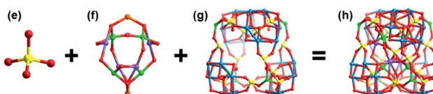
Fig. 1 Simplified (a–d) and real (e and h) three-shell nested subunit for NENU-605 . (a, e) The innermost shell (central PO 4 3- group); (b, f) the shuttle-shaped second shell ( \{Na_2K_4Mn_4\} ); (c, g) the cage-like outermost shell (Mn 4 (P 4 Mo 6 ) 4 ); (d, h) the overall three-shell nested substructure. Colour code: P yellow, O red, Na orange, K light purple, Mn green, and Mo light blue.
