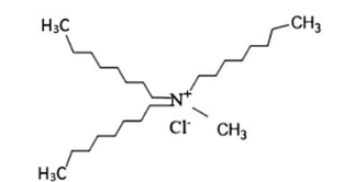
Molecular structure of MTOAC
