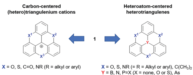
Fig. 2 Schematic representation of the carbon-centered triangulonium and heteroatom-centered triangulene derivatives deduced from the parent compound 1 .
