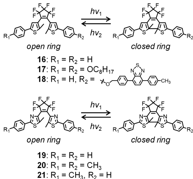
Fig. 6 Photochromism of diarylethene derivatives exhibiting dynamic crystal motions.
