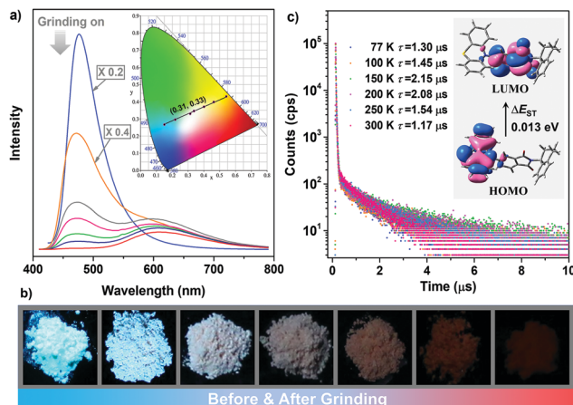
Fig. 5 Variations in emission properties of (S)-ImNT triggered by external force. (a) Changes of PL spectra of (S)-ImNT under grinding. “ \times 0.2 ” and “ \times 0.4 ” mean that intensities of the spectra presented in the figure are one fifth and two fifths of those of the original ones, respectively. The inset depicts linear changes of CIE_{x,y} coordinates of (S)-ImNT under grinding. (b) Luminescent images of the samples upon grinding treatments (under the illumination of 365 nm UV light). (c) Emission decay curves of the well-ground sample at different temperatures under vacuum. The insets are the Kohn–Sham frontier orbitals of (S)-ImNT in the most possible quasi-equatorial conformation.
