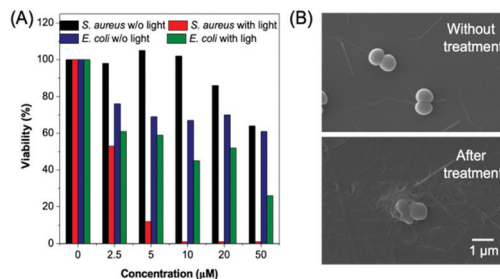
Fig. 7 Bacterial killing ability of BBR. (A) Statistical analysis of the bacterial viability data in Fig. S11 (ESI†). (B) SEM images of S. aureus incubated (upper picture) without treatment and (lower picture) with 10 \mu\text{M} BBR for 20 min, followed by 30 min of white light irradiation (60 \text{mW cm}^{-2} ). Scale bar: 1 \mu\text{m} .
