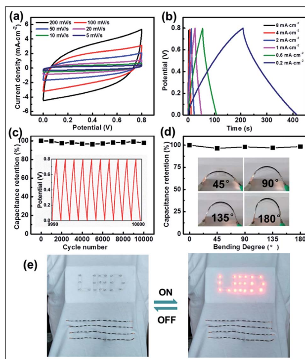
Fig. 5 (a) CV curves of micro-SCs based on CNB fibers in \text{H}_3\text{PO}_4 /PVA solid-state electrolyte, with scan rates increased from 5 to 10, 20, 50, 100 and 200 \text{ mV s}^{-1} . (b) GCD curves of micro-SCs, with current density increased from 0.2 to 0.6, 1, 2, 4 and 8 \text{ mA cm}^{-2} . (c) The cycling stability of micro-SCs at a voltage of 0.8 V at a current density of 0.4 \text{ mA cm}^{-2} ; the inset: GCD curves after 10 000 cycles between 0 and 0.8 V. (d) Capacitance retention of the CNB micro-SCs at different bending states at a current density of 0.4 \text{ mA cm}^{-2} . (e) Four CNB micro-SCs were connected in series into woven fabric and powered 19 LEDs.
