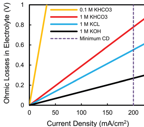
Fig. 4 Expected ohmic losses as a function of current density for commonly-used electrolytes in an electrochemical cell with a combined 3 mm catholyte and anolyte thickness at 25\text{ }^\circ\text{C} .
