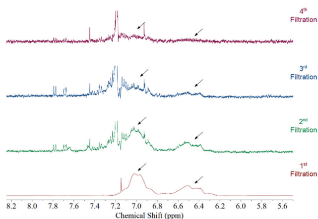
Fig. 1 NMR spectrum of the filtrates after each washing step of the functionalization procedure. This spectrum was taken from a sample where acetone was used as the solvent. The arrows point to the position of polystyrene aromatic protons. No polymer can be observed after the fourth redispersion.
