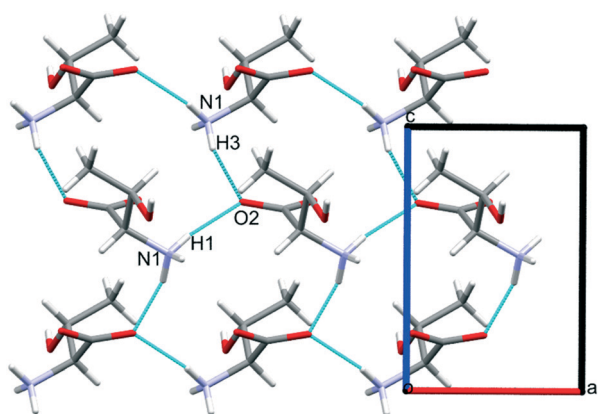
Fig. 6 Hydrogen bonding in L-threonine at ambient pressure as viewed along b .
