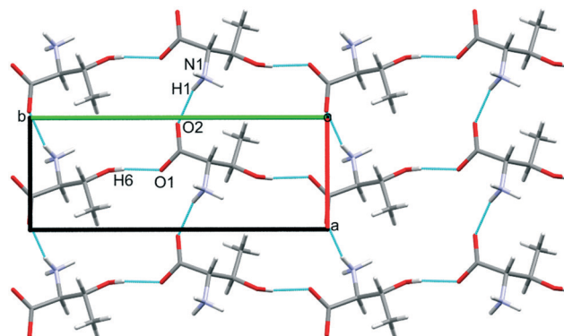
Fig. 5 Hydrogen bonding in L-threonine at ambient pressure, as viewed along c .
