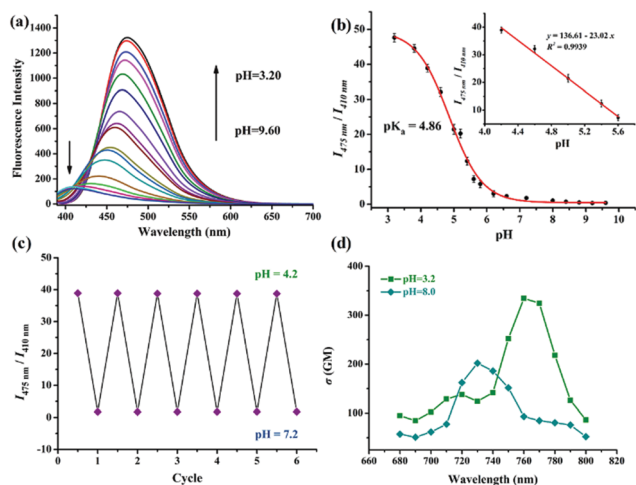
Fig. 1 (a) Emission spectra of Lyso-MPCB (10 \mu M) in B-R buffer solution with different pH from 9.60 to 3.20 (with 30% DMSO, \lambda_{\text{ex}} = 370 nm). (b) Plot of the fluorescence intensity ratio ( I_{475\text{nm}}/I_{410\text{nm}} ) vs. pH. Inset: Linear relationship of pH-dependent fluorescence intensity ratio ( I_{475\text{nm}}/I_{410\text{nm}} ). R^2 = 0.9939. (c) pH reversibility of Lyso-MPCB in B-R buffer solution (pH = 4.20 and 7.20). (d) Two-photon absorption cross-section of Lyso-MPCB with pH = 3.2 and 8.0, respectively. ( \lambda_{\text{ex}} = 680–800 nm).
