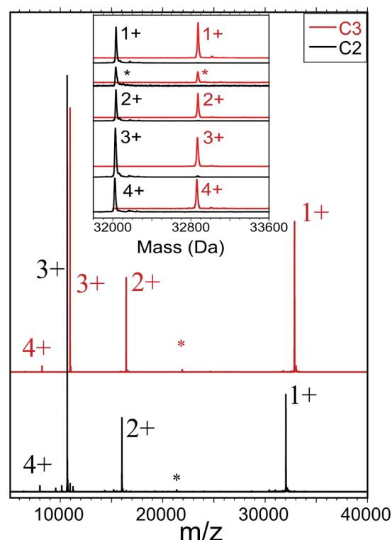
Fig. 1 Analysis of \text{Au}_{144}(\text{SC}_2)_{60} and \text{Au}_{144}(\text{SC}_3)_{60} by electrospray ionization mass spectrometry (ESI-MS). The main frame shows a complete mass spectrum for \text{Au}_{144}(\text{SC}_2)_{60} (in black) overlaid by a spectrum for \text{Au}_{144}(\text{SC}_3)_{60} (in red), spanning the mass-to-charge ( m/z ) range of 5000–40 000. Labels designate our assignments to charge states ( z = 1+, 2+, 3+ , and 4+ ) of the intact clusters or parent molecules, Mz^+ . The inset demonstrates the quantitative basis for these assignments by the alignment of all major features when the m/z -values are converted to mass ( m ) by multiplication of the respective portions of the spectrum by the assigned charge ( z ). For the minor features marked by the asterisk (*), the multiplier z = 3/2 is used, suggesting that these ions may arise from a dimer of the respective compounds in the z = 3+ charge-state, (2M)^{3+} . The so-determined masses agree with those calculated from the molecular formulas, within the instrumental precision. The mass-differences separating respective C2 and C3 principal peaks, are all 840–841 Da, in agreement with the count of 60 ligands, i.e. , the sixty additional methylene groups, ^{12}\text{C}^1\text{H}_2 , increment the mass by \sim 60 \times 14 = 840 Da.
