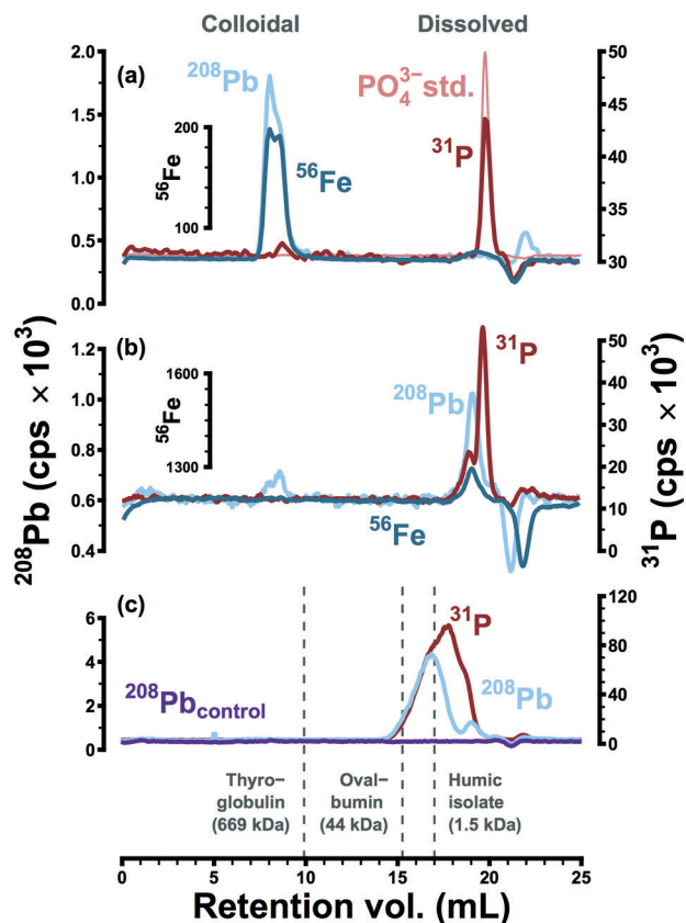
Fig. 1 (a) In system A size-separations (<0.05 mg P L -1 polyphosphate), ^{208}\text{Pb} eluted in a high molecular weight colloidal fraction—along with ^{56}\text{Fe} —while ^{31}\text{P} eluted in the same retention volume as the orthophosphate anion. (b) In system C size-separations (0.20 mg P L -1 polyphosphate), ^{208}\text{Pb} and ^{56}\text{Fe} eluted in a low molecular weight (dissolved) fraction along with ^{31}\text{P} and consistent with sequestration by polyphosphate. (c) ^{208}\text{Pb} and ^{31}\text{P} coeluted at low apparent molecular weight in deionized water with sodium hexametaphosphate, a strong complexing agent for lead. Peak retention volumes of thyroglobulin (hydrodynamic diameter: 17 nm), ovalbumin (diameter: 6 nm), and a Pb-tagged humic isolate are provided as qualitative points of reference.
