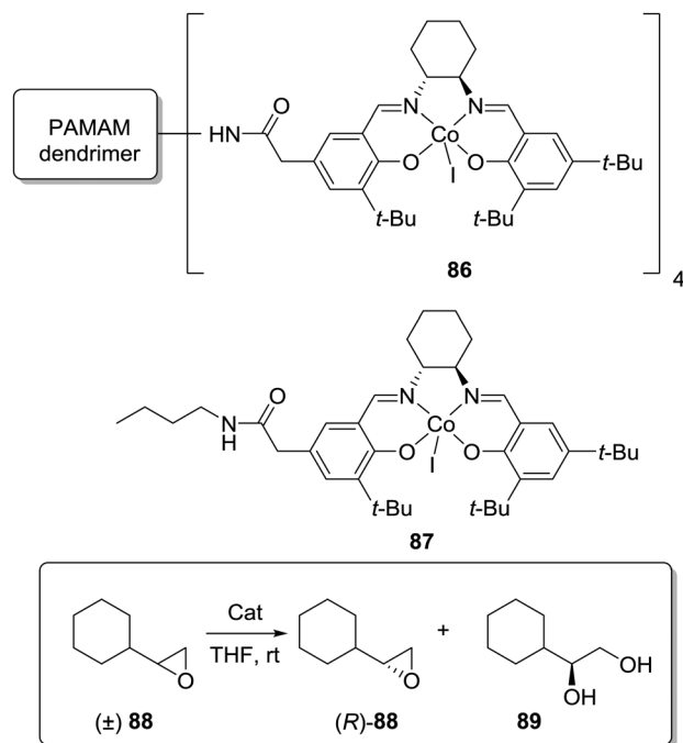
86 , Relative rate per [Co(Salen)] unit: 24, 99% ee 87 , Relative rate per [Co(Salen)] unit: 1, 98% ee
