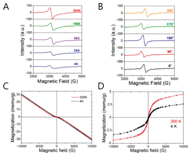
Fig. 7 (A) The temperature dependent EPR spectra of SOQS HgSe (B) angle dependent EPR spectra of SOQS HgSe (C) magnetization curves of HgSe CQD with different temperature (D) superparamagnetic curves with 300 and 4 K temperature. Adapted with permission from ref. 40. Copyright 2017 American Chemical Society.
