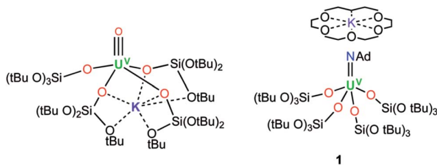
Fig. 1 Molecular structures of the U V terminal oxo complex, [UO{OSi(OtBu) 3 } 4 K] (left), and the U V terminal imido complex, [K(18c6)][U(NAd){OSi(OtBu) 3 } 4 ] (1) (right).
