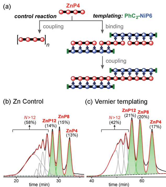
Fig. 10 Reaction design and outcome of linear Vernier templating for the synthesis of \text{ZnP12} from \text{ZnP4} using \text{PhC2-NiP6} as a template. (a) Reaction scheme. (b) GPC traces (detection at 591 nm, toluene/1% pyridine) of the non-templated reaction and (c) the templated reaction product mixture after removal of the template \text{PhC2-NiP6} at 4 h. Products were identified by analytical GPC based on calibrated retention times. 19 The percentages in GPC traces are the analytical yields of each oligomer, from integration of the peaks (absorption at 591 nm).
