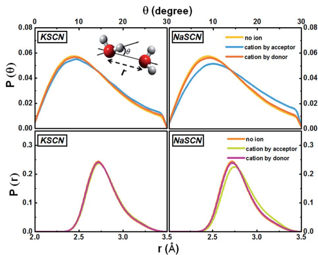
Fig. 5 Distributions of the water–water hydrogen bonding angle and distance in the 0.5 M KSCN and NaSCN solutions. The inset of the upper left panel gives the definitions of these two geometrical parameters. When a cation appears next to the acceptor water, both distributions deviate from the non-ion case. In the NaSCN solution, this deviation is much more significant (note that this does not suggest that the \text{Na}^+ hydration shell is more distorted than that of \text{K}^+ , see Section G of the ESI† for a further discussion).
