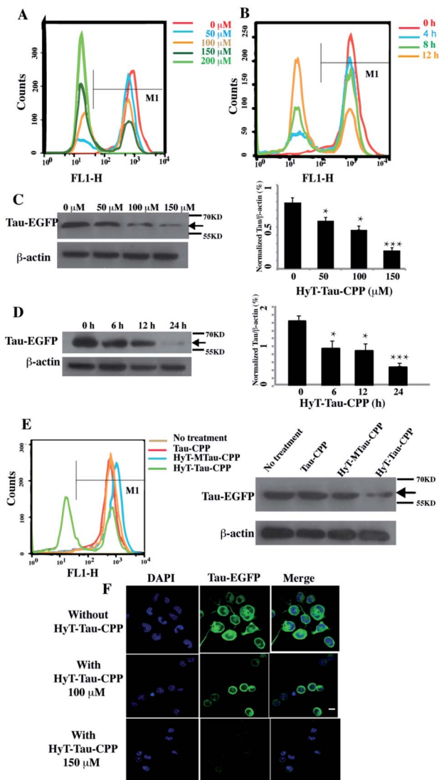
Fig. 3 HyT-Tau-CPP can lead to the degradation of intracellular Tau effectively. (A) The flow cytometry results of the Tau-EGFP overexpressed cells with the treatment of 0 μM, 50 μM, 100 μM, 150 μM, 200 μM of HyT-Tau-CPP for 24 h. The gray horizontal line represents the fluorescence positive signal threshold. (B) The flow cytometry results of the Tau-EGFP overexpressed cells with the treatment of 150 μM HyT-Tau-CPP for different time. The gray horizontal line represents the fluorescence positive signal threshold. (C) Representative western blot results for Tau and β-actin revealed a concentration-dependent degradation of Tau treated with 0 μM, 50 μM, 100 μM, 150 μM HyT-Tau-CPP for 24 h. Values for all Tau and β-actin are mean ± SD ( n = 3 independent experiments). The level of Tau is measured by densitometry and normalized with β-actin level. Statistical significance compared to the control (0 μM) was analyzed by one-way ANOVA, * P < 0.05 , ** P < 0.01 , *** P < 0.001 . (D) Representative western blot results for Tau and β-actin revealed a time-dependent knockdown of Tau with the treatment of 150 μM HyT-Tau-CPP for 0 h, 6 h, 12 h, 24 h in the same cell line. Values for all Tau and β-actin are mean ± SD ( n = 3 independent experiments). The level of Tau is measured by densitometry and normalized with β-actin level. Statistical significance compared to the control (0 h) was analyzed by one-way ANOVA, * P < 0.05 , ** P < 0.01 , *** P < 0.001 . (E) The flow cytometry and western blot for Tau and β-actin results of the Tau-EGFP overexpressed cells with the treatment of 150 μM Tau-CPP, 150 μM HyT-MTau-CPP, 150 μM HyT-Tau-CPP or vector for 24 h. The results demonstrated that the Tau-CPP and HyT-MTau-CPP couldn't
