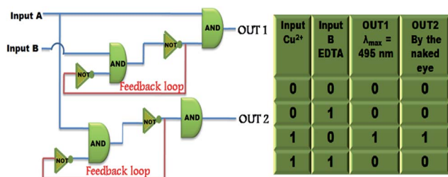
Fig. 9 Truth table and sequential logic circuits displaying memory units with two inputs (input A (Cu 2+ ) and input B (EDTA)) and two outputs in the presence of chemical inputs.
