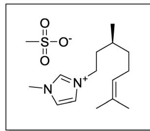
Scheme 1 Structure of the (S)-(3,7-dimethyloct-6-en-1-yl)-1-methyl-1 H -imidazol-3-ium methanesulfonate.
