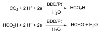
Scheme 8 Electrocatalytic reduction with boron doped-diamond electrodes with highest efficiency for formaldehyde at -1.7 \text{ V} . 16
