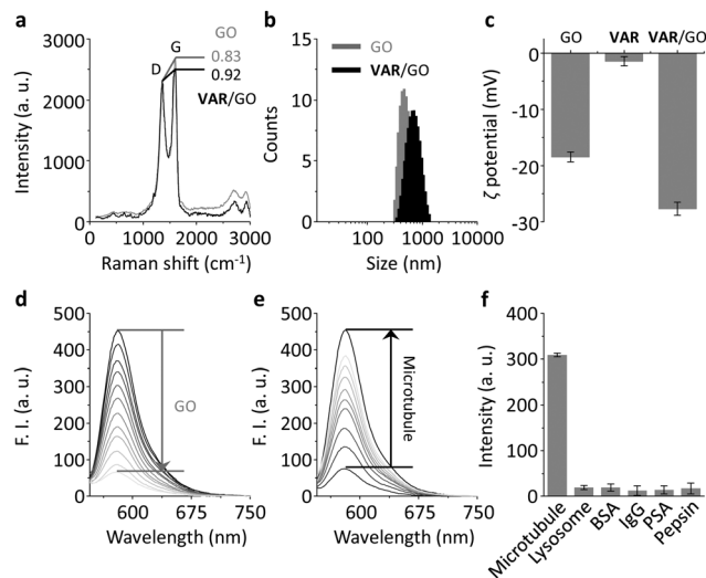
Fig. 2 (a) Raman spectroscopy of GO (30 \mu\text{g mL}^{-1} ) and VAR/GO (1.5 \mu\text{M} /30 \mu\text{g mL}^{-1} ). (b) Dynamic light scattering of GO (9.1 \mu\text{g mL}^{-1} ) and VAR/GO (0.5 \mu\text{M} /9.1 \mu\text{g mL}^{-1} ). (c) Zeta ( \zeta ) potential of VAR probe (0.5 \mu\text{M} ), GO (9.1 \mu\text{g mL}^{-1} ) and VAR/GO (0.5 \mu\text{M} /9.1 \mu\text{g mL}^{-1} ). (d) Fluorescence spectra of VAR probe (0.5 \mu\text{M} ) in the presence of increasing GO (0–9.1 \mu\text{g mL}^{-1} ). (e) Fluorescence spectra of VAR/GO (0.5 \mu\text{M} /9.1 \mu\text{g mL}^{-1} ) in the presence of increasing microtubule (0–29.56 nM). (f) Fluorescence intensity of VAR/GO (0.5 \mu\text{M} /9.1 \mu\text{g mL}^{-1} ) in the presence of microtubule (29.56 nM) and other proteins (30 nM) (BSA = bovine serum albumin; PSA = pisin sativum agglutinin; IgG = immunoglobulin G). All fluorescence measurements were carried out in phosphate buffered saline (0.01 M, pH 7.4) at room temperature with an excitation wavelength of 510 nm.
