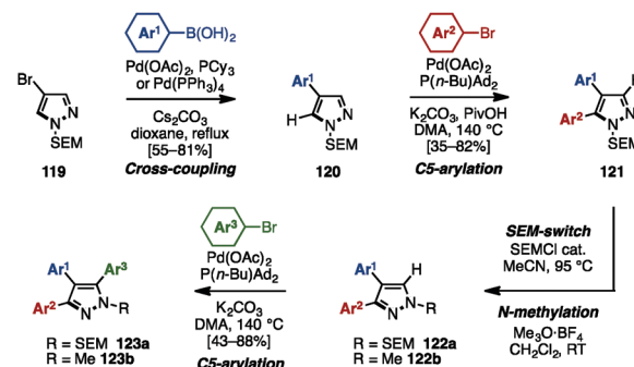
Scheme 21 Regioselective sequential C–H arylation of SEM-protected pyrazoles.
