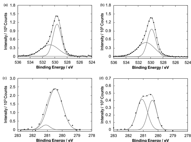
Fig. 7 O\ 1s XPS spectra of the Ru–ZnP/TiO 2 /FTO electrodes (a) before and (b) after the PEC operation. Ru 3d_{5/2} XPS spectra of the Ru–ZnP/TiO 2 /FTO electrodes (c) before and (d) after the PEC operation.
