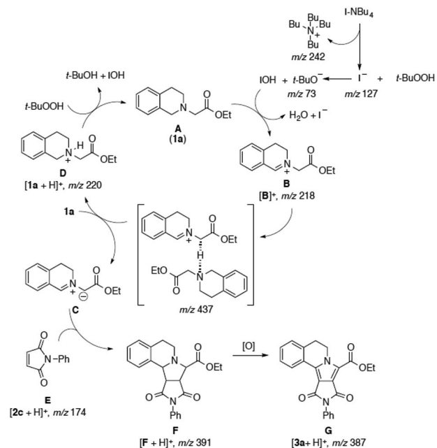
Scheme 1 Proposed mechanism.
