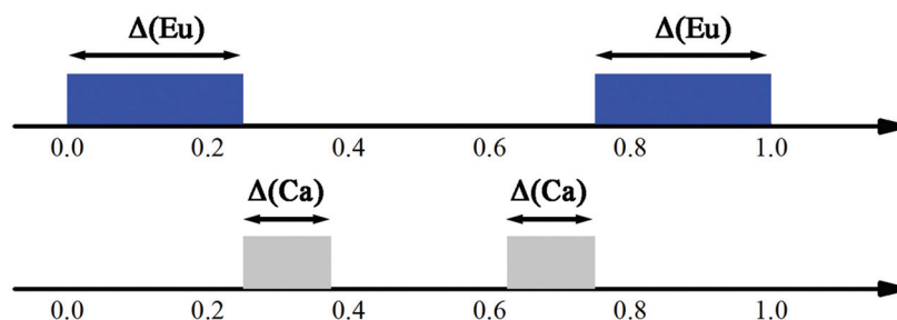
Fig. 7 Schematic view of the crenel domains in the superspace. The Eu domain (blue) is centered at x_4^0 = 0 with \Delta = 1/2 . Two crenel domains of Ca (grey) are centered at x_4^0 = 5/16 and 11/16 with \Delta = 1/8 , respectively. Reproduced with permission from ref. 66. Copyright 2013 American Chemical Society.
