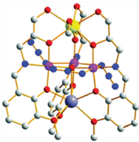
Fig. 20 Structure of the heterometallic [\text{Mn}_{13}\text{CaNa}] cluster 39 . Hydrogen atoms are omitted for clarity. Color code: blue (N), large, dark-gray (Na), gray (C), red (O), violet (Mn), and yellow (Ca). Adapted from ref. 143 with permission from the Royal Society of Chemistry.
