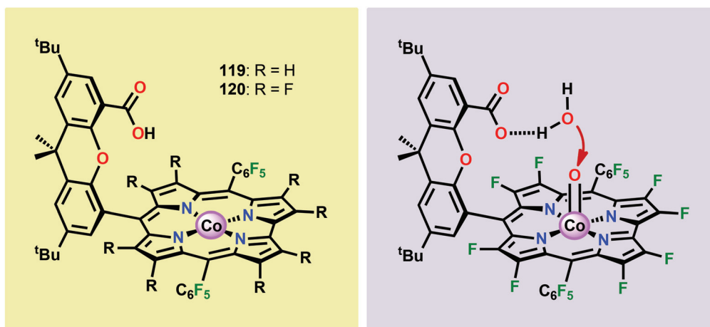
Fig. 43 (Left) Co corrole complexes 119 and 120 , and (right) organization of \text{H}_2\text{O} within the Co hangman cleft.
