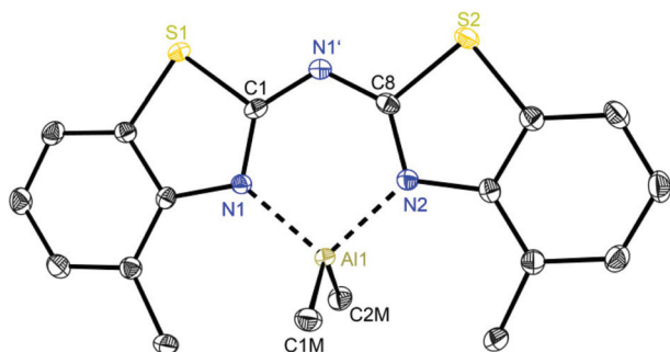
Fig. 6 Molecular structure of [\text{Me}_2\text{Al}(\{4\text{-MeNCSC}_6\text{H}_3\}_2\text{N})] ( 5 ). Anisotropic displacement parameters are depicted at the 50% probability level. Hydrogen atoms are omitted for clarity. Structural data are given in Tables 1 and 3.
