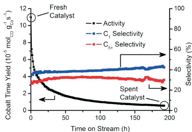
Fig. 2 Catalytic activity and selectivity towards methane (C 1 ) and higher hydrocarbons (C 5+ ) during the first 200 h of FTS reaction (250 °C, 1 bar, H 2 /CO = 2).
