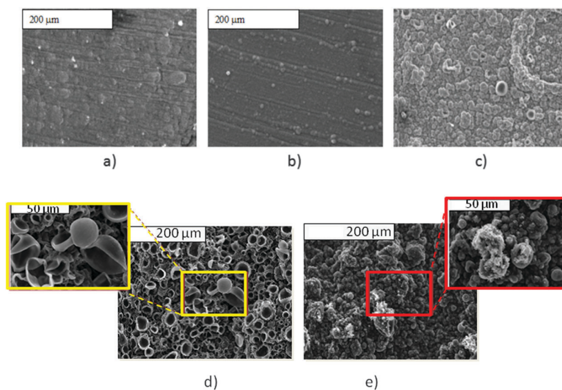
Fig. 6 S.E.M. studies of PPy films doped with different anions: (a) PPy(CIO 4 ); (b) PPy(DBS); (c) PPy( 1 ) and its surface modification by [NBu 4 ] + and [PBU 4 ] + , (d) and (e) respectively. (Fig. 6d reproduced with permission from ref. 8. Copyright 2002, John Wiley and Sons).
