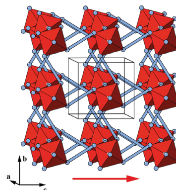
Fig. 12 Representation of a hypothetical polar Pma2 molecular perovskite phase, where the polarisation is indirectly induced via superposition of shift and tilt distortions. Here the blue rods signify molecular bridging units of indeterminate composition. The polarisation direction is indicated by the red arrow.
