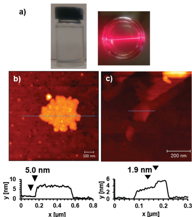
Fig. 2 (a) Images showing a suspension of \text{Cu}(1) nanosheets in DMF with characteristic Tyndal Scattering of laser light. AFM images and height profiles corresponding to blue lines for nanosheets formed by exfoliation of (b) \text{Zn}(1) in DMF (c) \text{Cu}(1) in \text{H}_2\text{O} .
